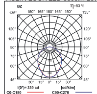
RUBIN LOOK LED 3300lm 25W MICRO-PRM E IP44
